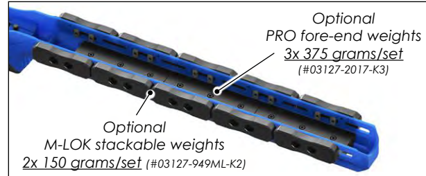
Fore-end with built-in Arca Elite System (AES) - Bottom view
