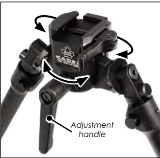
FALCON LITE AES BIPOD - Part#: 7431-K102AES
