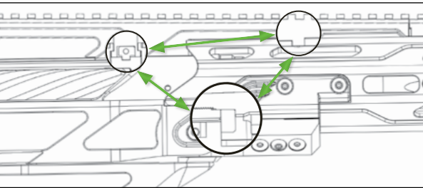
Triple recoil lug system
